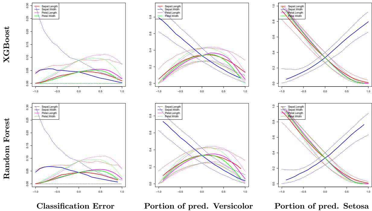
Figure 2: Evaluation of the classification error and the prediction \tau with respect to the explanatory variable perturbation \tau , on the Iris dataset (Section 4.2). The quantity \tau and the plain/dashed lines have the same signification as in Fig. 1. (Top) XGBoost Model. The sepal width enables to differentiate the Setosa class. (Bottom) Random Forest Model. The sepal width again enables to differentiate the Setosa class.
