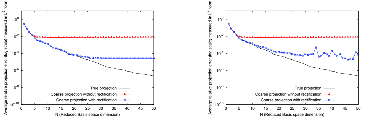
Figure 5: Average errors with \lambda = 10^{-10} (left) and with \lambda = 0 (right) during the reduced basis construction stage with \Xi_{train} = \Xi_{train}^F
