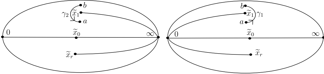
FIGURE 2. Domain of definition of \tilde{\Phi}_0^d(z) (left) and \tilde{\Phi}_\infty^d(z) (right).
