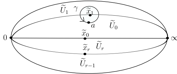
FIGURE 3. Domain of definition of \tilde{P}^d .
