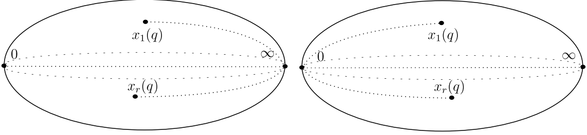
FIGURE 1. Intersection of \bar{S}(d - \frac{\pi}{2k}, d + \frac{\pi}{2k}) and the domain of definition of \Phi_0^{[d]}(z, q) (left) and \Phi_\infty^{[d]}(z, q) (right).
