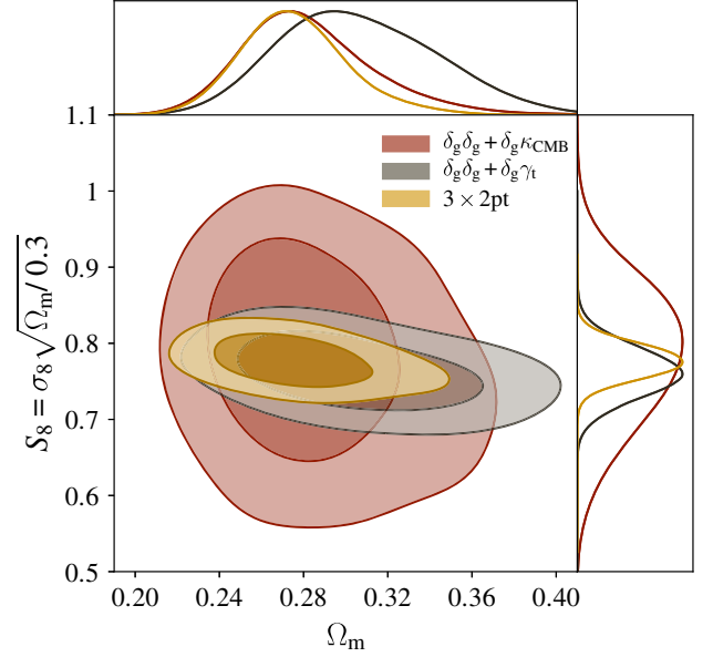
FIG. 6. Constraints on \Omega_m and S_8 from the measurements of this paper and combinations of other two-point correlation functions. We show the constraints from w^{\delta_g\delta_g}(\theta) + w^{\delta_g\kappa_{\text{CMB}}}(\theta) (red), w^{\delta_g\delta_g}(\theta) + w^{\delta_g\gamma_t}(\theta) (gray) and 3 \times 2 point (gold).
