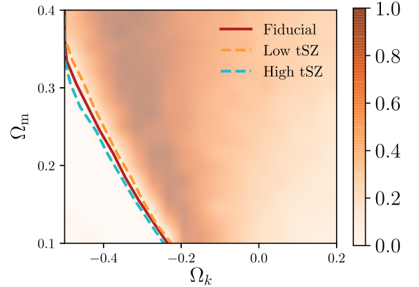
Figure 5. The constraints on \Omega_m and \Omega_k resulting from analysis of the measured lensing ratios. The background colour shows the marginalized posterior density for these two parameters. The data strongly rule out regions of parameter space with low \Omega_m and very negative \Omega_k . At each \Omega_m , we identify a lower limit on \Omega_k by identifying the value of \Omega_k for which the marginalized posterior falls by 1/e^2 relative to the maximum, which for a Gaussian distribution would correspond to the 2\sigma lower limit. This limit is illustrated with the red solid curve. We also show (dashed curves) the changes to these limits when using two variations on the fiducial tSZ model, as described in Section 4.3.
