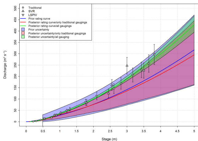
Figure 7. Stage–discharge rating curves and their uncertainty for the Auzon station: blue, prior rating curve based on hydraulic analysis only (no gaugings); red, rating curve established with traditional gaugings only; green, rating curve established with all gaugings, including high-flow non-contact gaugings. Solid lines represent the rating curves. Shaded areas represent the corresponding uncertainty 95 % confidence intervals.
