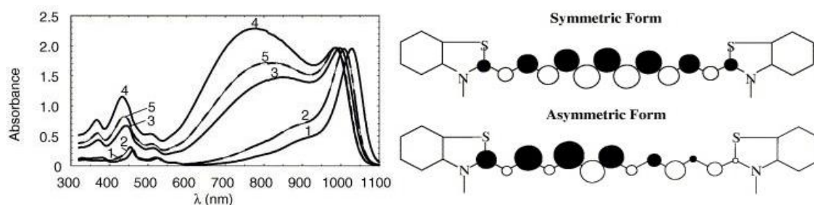
Figure 6. Absorption spectra of undecamethine reported by Lepkowicz et al. (left) in o -dichlorobenzene (1), dichloromethane (2), ethanol (3), acetonitrile (4) and methanol (5). Determined symmetric and asymmetric forms (right). Figure adapted from ref. [41].
