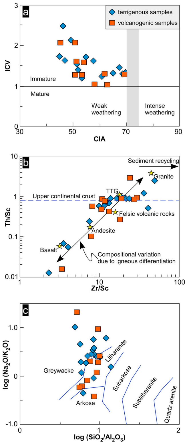
Figure 4. Geochemical characteristics of Ordovician sedimentary rocks from the Mongolian Altai. (a) CIA-ICV classification diagram after Nesbitt and Young (1984) and Cox et al. (1995). (b) Zr/Sc versus Th/Sc diagram after McLennan et al. (1993). (c) Classification diagram after Pettijohn et al. (1987), showing the graywacke-dominated nature of the analyzed samples.
