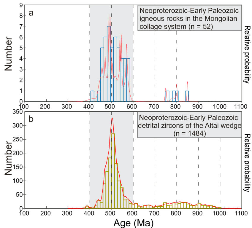
Figure 12. (a) Histogram of formation ages for Neoproterozoic-early Paleozoic (meta)igneous rocks from the Mongolian collage system (Xiao et al., 2015). Data are from Jiang et al. (2011, and references therein). (b) Histogram of ages for igneous-related Neoproterozoic-early Paleozoic detrital zircons from the Ordovician sedimentary succession of the Altai. Data sources are the same as in Figure 11.
