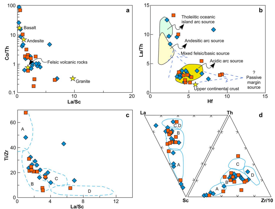
Figure 10. Source rock and tectonic setting discrimination diagrams for the Ordovician sedimentary succession from the Mongolian Altai. (a) La/Sc versus Co/Th diagram (after Condie et al., 1992; Gu et al., 2002; McLennan et al., 1984), showing derivation mainly from mixed felsic-intermediate volcanic source. (b) Hf versus La/Th diagram (after Floyd & Leveridge, 1987), indicating predominantly felsic sources. (c) La/Sc versus Ti/Zr diagram (after Bhatia & Crook, 1986), suggesting a continental arc and active continental margin setting. (d) Triangular trace element plots (after Bhatia & Crook, 1986) suggesting a continental island arc/active continental margin affinity. A = oceanic island arc; B = continental island arc; C = active continental margin; D = passive margin.
