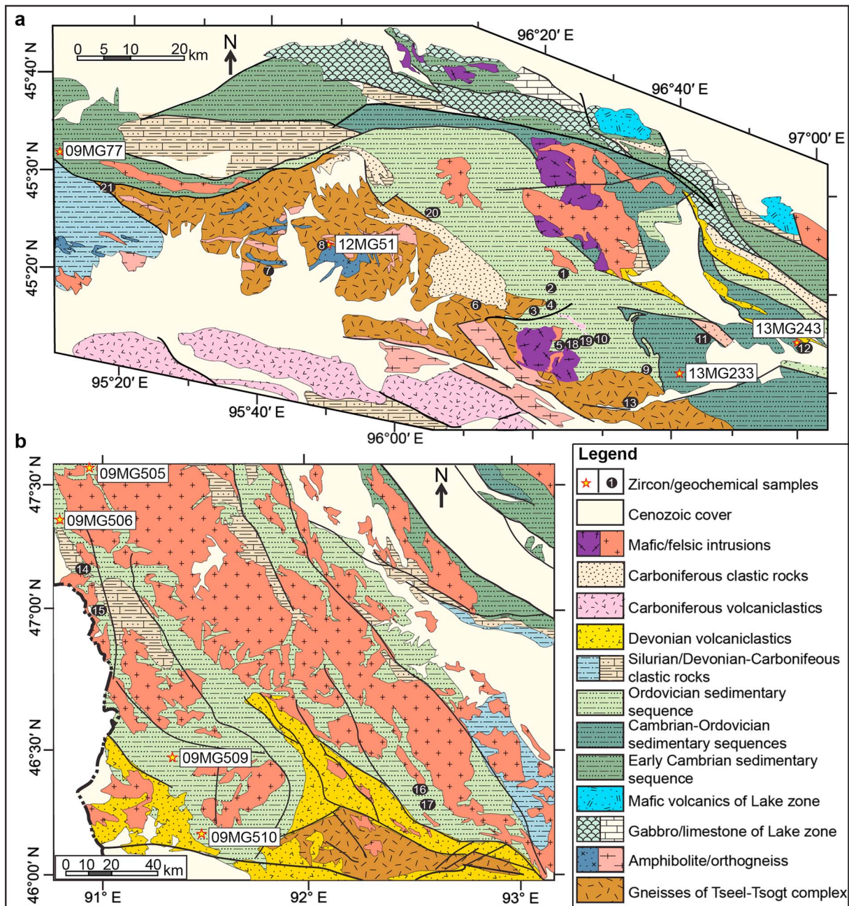
Figure 2. Geological map of the studied areas in SW Mongolia. Modified from Tomurtogoo (1998) and Hanžl et al. (2016). Sample locations are shown. Numbers in circles refer to samples in numerical order in Table S1. See Figure 1 for location of the figures.
