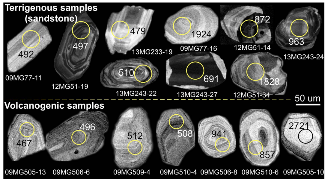
Figure 6. Representative CL images of zircons from samples of terrigenous-volcanogenic sedimentary succession of the Mongolian Altai. Analytical positions and ages (Ma) are labeled, and analysis numbers as in Table S2 are also indicated.
