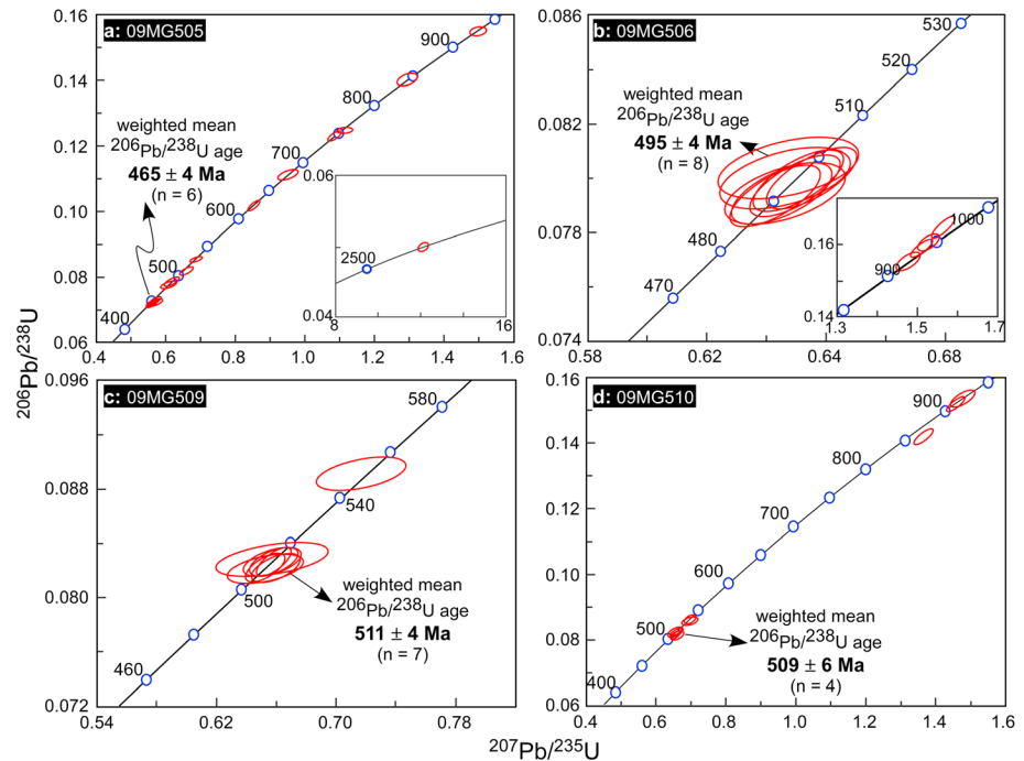
Figure 8. U-Pb concordia diagrams for zircons from volcanogenic rocks of the Ordovician succession in the Mongolian Altai.
