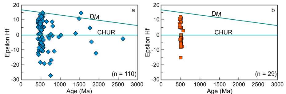
Figure 9. Diagrams of \epsilon_{\text{Hf}}(t) values versus crystallizing ages for zircons from (a) terrigenous and (b) volcanogenic samples of the Ordovician succession. Age data with discordance larger than 10% are excluded.
