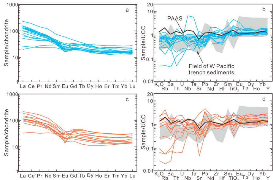
Figure 5. Chondrite-normalized REE and upper continental crust (UCC) normalized trace element patterns for (a, b) terrigenous and (c, d) volcanogenic samples. Normalizing values are from Sun and McDonough (1989) and Taylor and McLennan (1985), respectively. Literature data for Pacific-type trench sediments of Plank and Langmuir (1998) and the average post-Archean Australian shale (PAAS) of Taylor and McLennan (1985) are shown for comparison.
