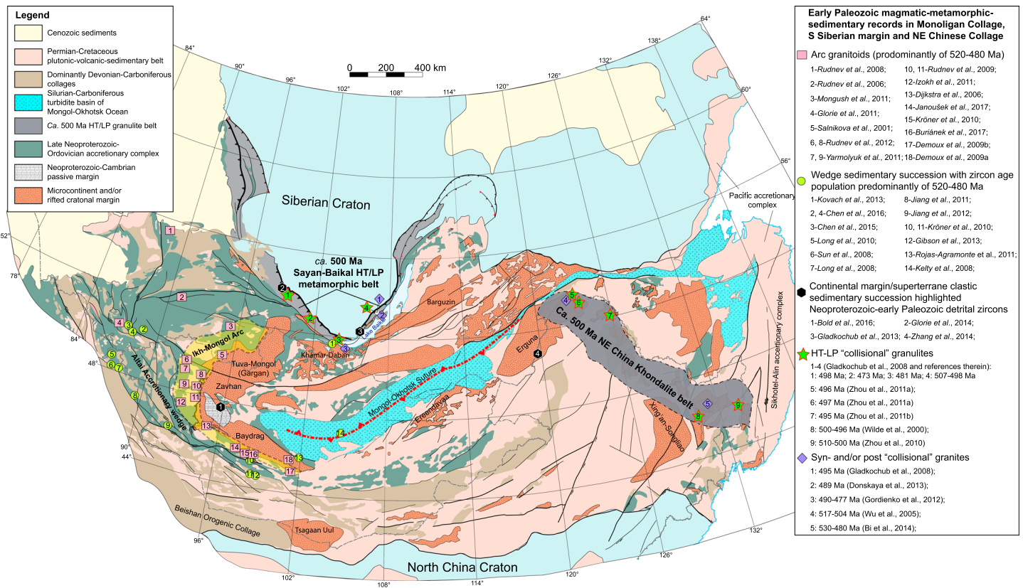
Figure 14. Simplified tectonic map of the eastern CAOB showing spatial distribution of major superterrane belts, circa 500 Ma HT/LP granulitic metamorphic belt along margins of Siberian Craton and the Khondalite belt in NE China as well as the Altai accretionary system including Cambro-Ordovician Ikh-Mongol magmatic arc system (highlighted) and Altai accretionary wedge. Published zircon U-Pb data related to the early Paleozoic magmatic-metamorphic records in the Mongolian collage system, south Siberian margin, and NE Chinese collage are also indicated.
