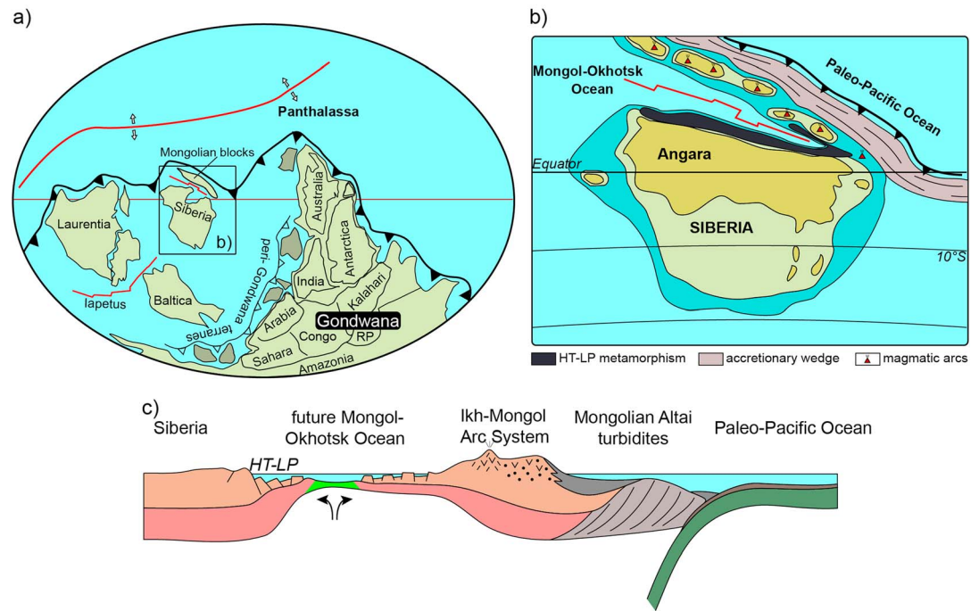
Figure 15. (a) Updated geodynamic scenario placing the Mongolian CAOB into a paleo-Pacific subduction system that extended from the TAO of NE Gondwana to Siberia. Global paleogeographic reconstructions in the Late Cambrian (circa 500 Ma) are modified from Scotese (2001). (b, c) Geodynamic model explaining the development of a typical HT/LP Baikalian granulitic metamorphic belt and a peri-Pacific Altai accretionary system, respectively. See text for details.
