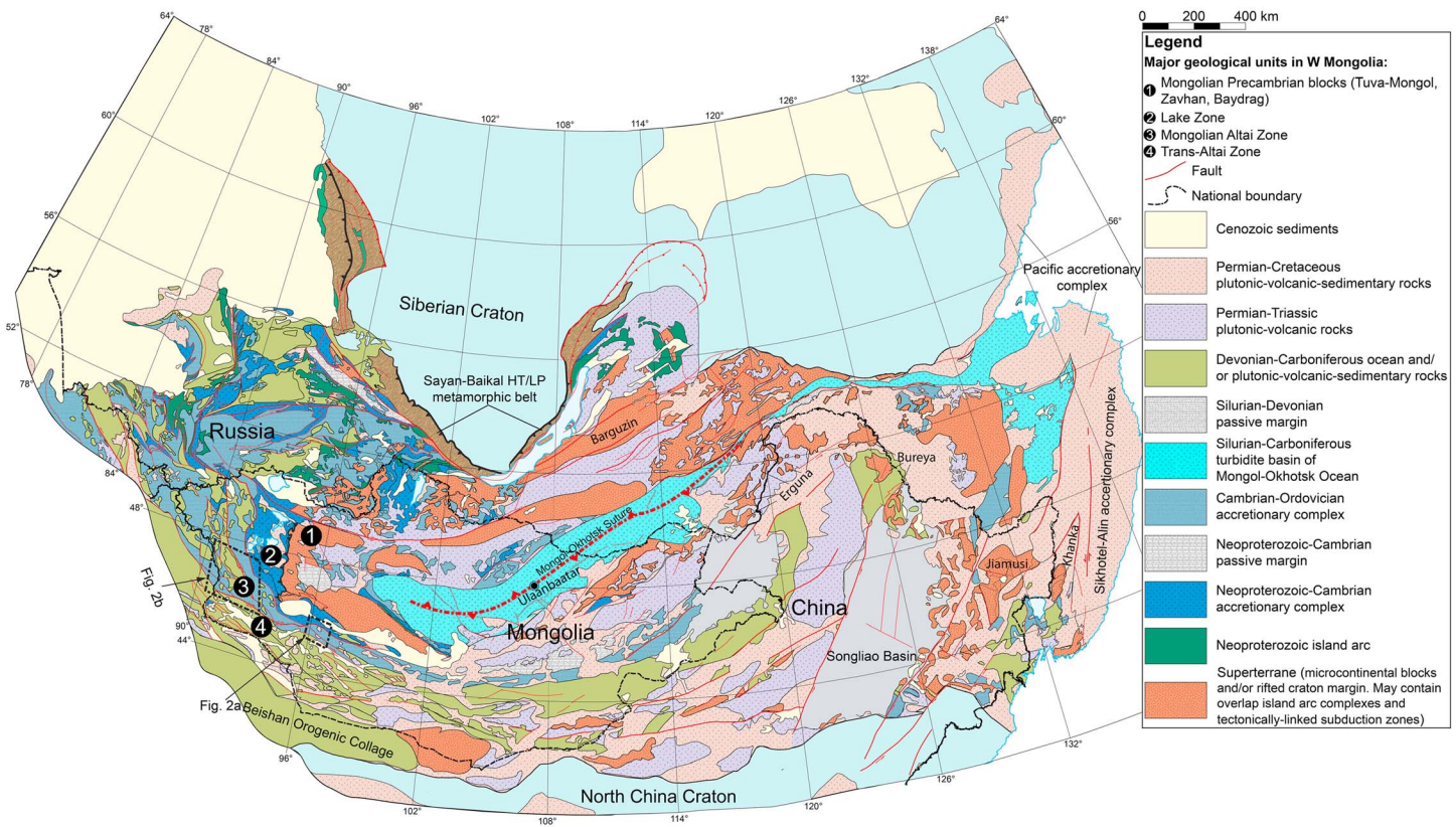
Figure 1. Simplified geological map of the central CAOB (modified from Parfenov et al., 2003). Positions of major units in western Mongolia and the studied areas are also indicated.
