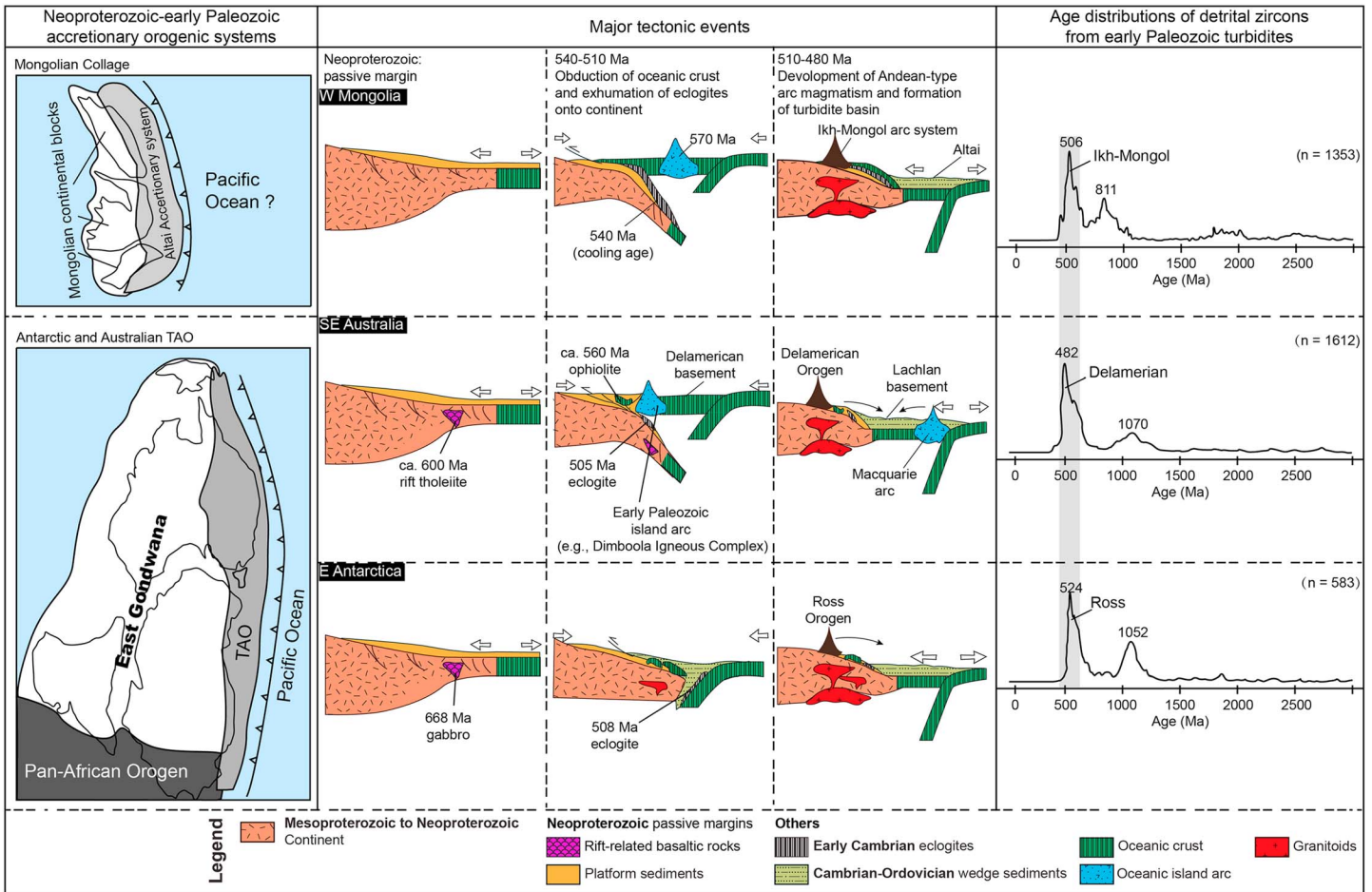
Figure 13. Architecture and main tectonic cycles of the accretionary system of the Mongolian collage system compared with that of the TAO. See text for detailed explanation. Detrital age patterns of zircons from early Paleozoic sedimentary successions within these two systems are also presented for comparison. For Mongolian data sources, see Figure 11b. Data for the SE Australian TAO are from Ireland et al. (1998), Fergusson and Fanning (2002), Fergusson et al. (2005, 2007, 2013), Squire et al. (2006), and Glen et al. (2011), and data for East Antarctica are from Goodge et al. (2002, 2004).
