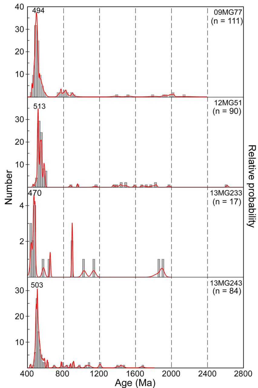
Figure 7. Relative probability plots for detrital zircon ages of terrigenous clastic sedimentary samples from the Ordovician succession. ^{206}\text{Pb}/^{238}\text{U} and ^{207}\text{Pb}/^{206}\text{Pb} ages are used for zircons younger and older than 1.0 Ga, respectively. Only analyses less than 10% discordant are considered in the plots to achieve the best possible age resolution (disc % = \text{abs}(100 - 100 \times (^{206}\text{Pb}/^{238}\text{U age}) / (^{207}\text{Pb}/^{206}\text{Pb age})) ), Gehrels (2012)). Determination of age peaks was done by ISOPLOT.
