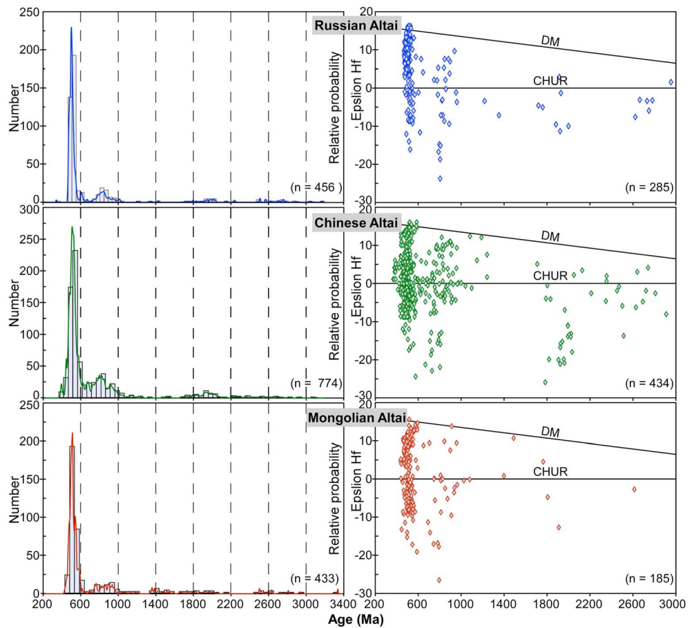
Figure 11. Age distribution and the Hf isotope pattern for igneous-related detrital zircons in Cambrian-Ordovician meta-sedimentary succession of the Russian Altai (data from Chen, Sun, Buslov, et al., 2015; Chen et al., 2016; Chen, Sun, Cai, et al., 2015), the Chinese Altai (data from Long et al., 2007, 2010; Sun et al., 2008; Jiang et al., 2011; Wang et al., 2014), and the Mongolian Altai (data from this study and previous works Jiang et al., 2012). ^{206}\text{Pb}/^{238}\text{U} ages are used for the grains younger than 1.0 Ga, and ^{207}\text{Pb}/^{206}\text{Pb} ages are used for the grains older than 1.0 Ga. We rely only on analyses that are less than 10% discordant.
