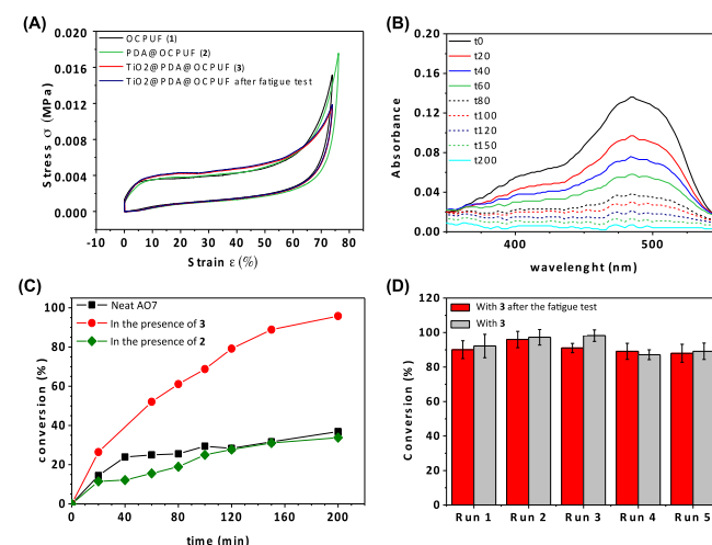
Fig. 4 (A) Stress/strain responses of 1 (black), 2 (green), as-synthesized 3 (red) and fatigue-tested 3 (blue). (B) UV-visible spectra of the AO7 solution vs. UV irradiation time (min) in the presence of 3 . (C) Degradation of AO7 (%) vs. UV irradiation time (min) for neat AO7 (black horizontal squares), AO7 with 2 (green squares), and AO7 with 3 (red dots); at least two runs have been performed in each case. (D) Degradation of AO7 (%) after 200 min UV irradiation for runs 1 to 5 with as-synthesized 3 (grey histograms) and fatigue-tested 3 (red histograms); the average value and standard deviation of at least three experiments are represented.
