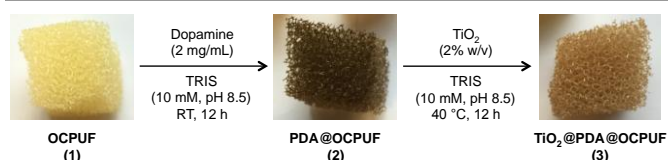
Fig. 2 Polyurethane open cell foam (OCPUF) coating with polydopamine (PDA) and functionalization with TiO 2 nanoparticles
