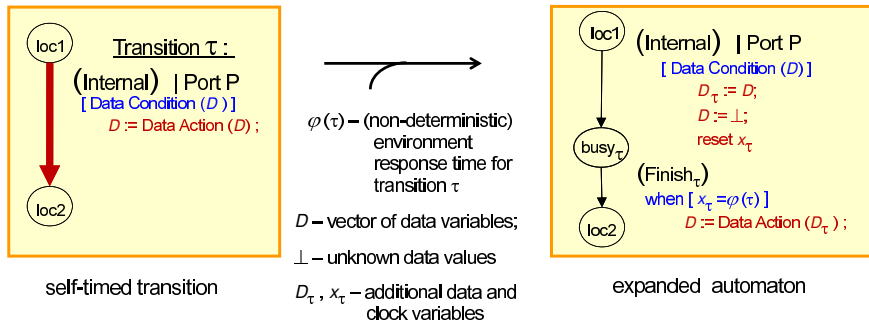
Fig. 6: Modeling tasks in BIP
