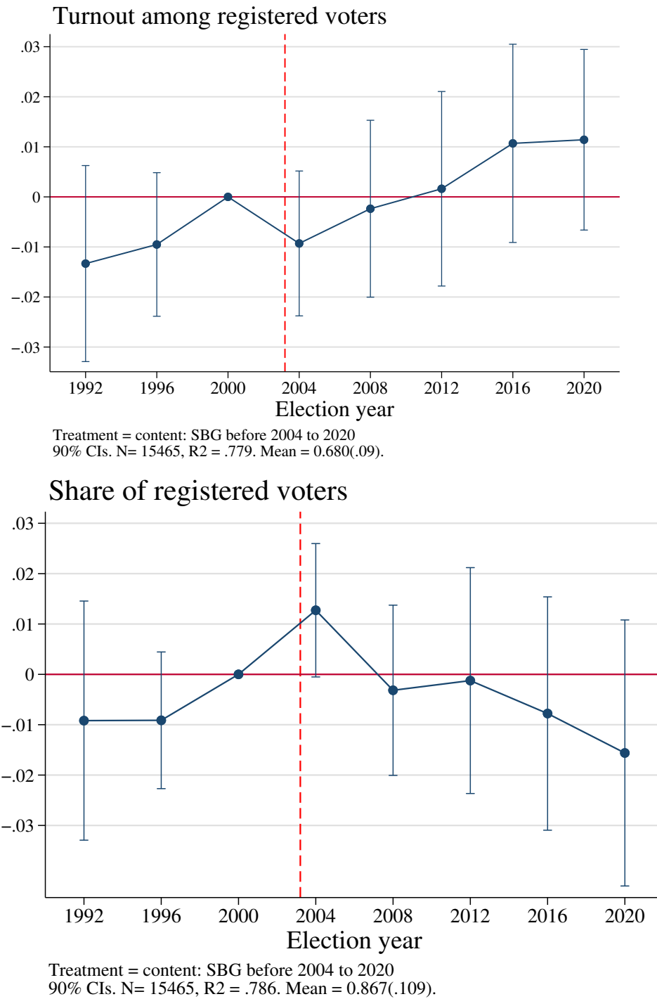
Fig. 6. Within county change in the turnout rate and the share of registered voters
