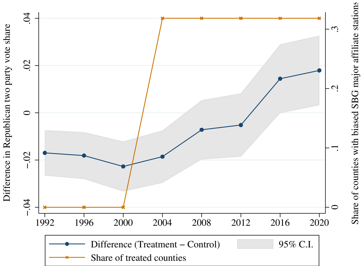
Fig. 3. Trend in the naive difference
