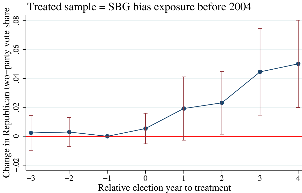
Fig. A1. Dynamic effect graph: Within county change in the Republican two-party vote share for president
