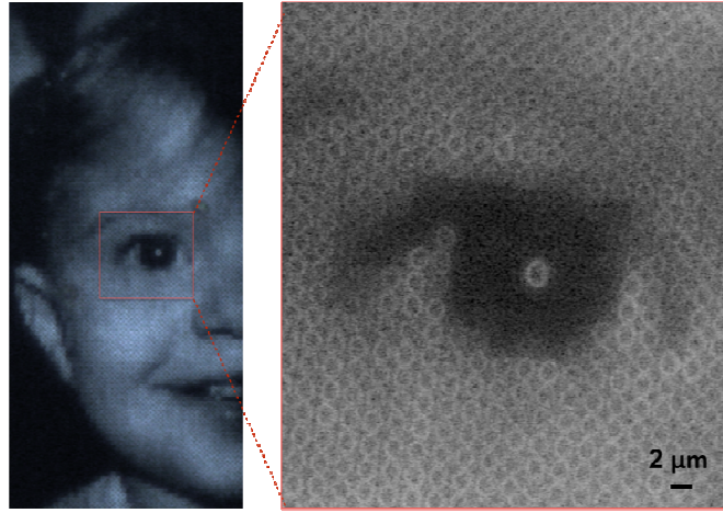
Figure 7. Optical data storage of a selected 200 \times 200 image encoded on 256 gray levels (not shown here): (left) encoded image as a 200 \times 200 pixels image on 256 gray levels of fluorescence emission under UV excitation ( \lambda_{\text{exc.}} = 365 \text{ nm} ), being partially recorded by wide-field fluorescence microscopy (objective 50\times , \text{NA} = 0.75 ); (right) zoom of a region of interest. The pixels consist of fluorescent rings with 1.6 \mu\text{m} diameters and 7 \mu\text{m} depth, equally positioned in a square lattice with 2 \mu\text{m} spacing.
