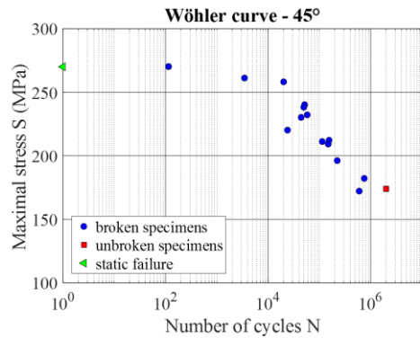
Fig. 11 : Wöhler curve at 45°
