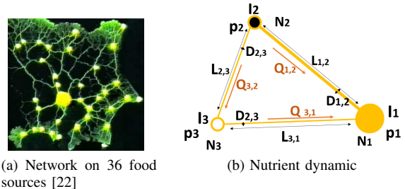
Fig. 1: Physarum network.
