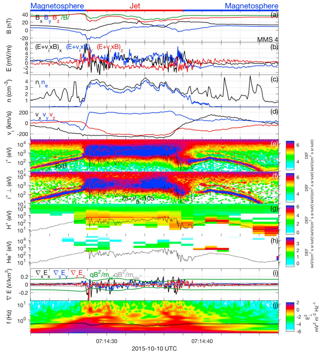
Figure 4. MMS4 observations of event 3 (10 October 2015) in GSE coordinates. (a) Magnetic field. (b) Electric field in the plasma frame ( \mathbf{E}+\mathbf{v}_i \times \mathbf{B} ). (c) Ion (black) and electron (blue) densities. (d) Ion bulk velocity. (e) Omnidirectional ion differential energy flux. Black, blue, and red lines correspond to \mathbf{E} \times \mathbf{B} energy for protons, \text{He}^+ , and \text{O}^+ , respectively. (f) Perpendicular ion differential energy flux. Black, blue, and red lines correspond to \mathbf{E} \times \mathbf{B} energy for protons, \text{He}^+ , and \text{O}^+ , respectively. (g) HPCA ion energy flux for protons (subspin resolution). (h) HPCA ion energy flux for \text{He}^+ (subspin resolution). (i) Electric field gradient calculated using four spacecraft. (j) Perpendicular \mathbf{E} field power wavelet spectrogram. f_{ci} is plotted in black.
