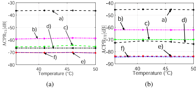
Fig. 20. ACPR performance of various adaptive DPDs: a) PA output, b) stand-alone LMS-ILA-based DPD, c) stand-alone RLS-ILA-based DPD, d) Design+LMS, e) Design+RLS, and f) PA input. (a) ACPR U1 . (b) ACPR U2 .
