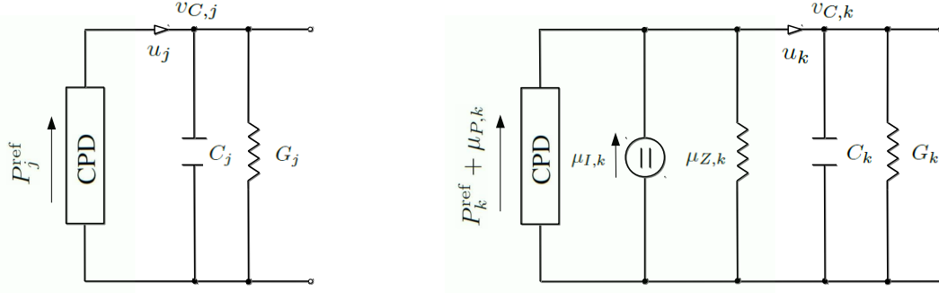
(a) Equivalent circuit scheme for PQ units.
