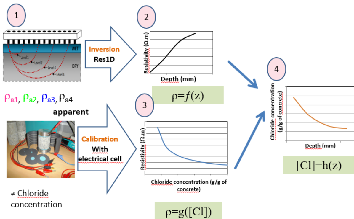
155 156 Figure 1 Schematic representation of the methodology used to obtain chloride content profiles in concrete
