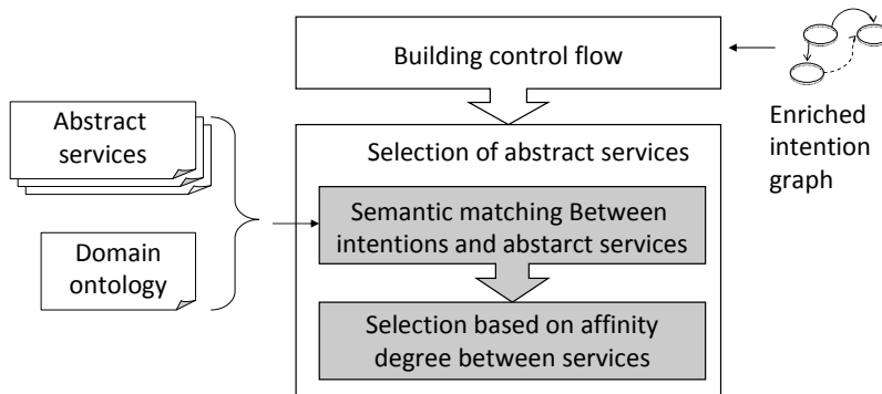
Figure 9: Steps of initial composition schema generation
