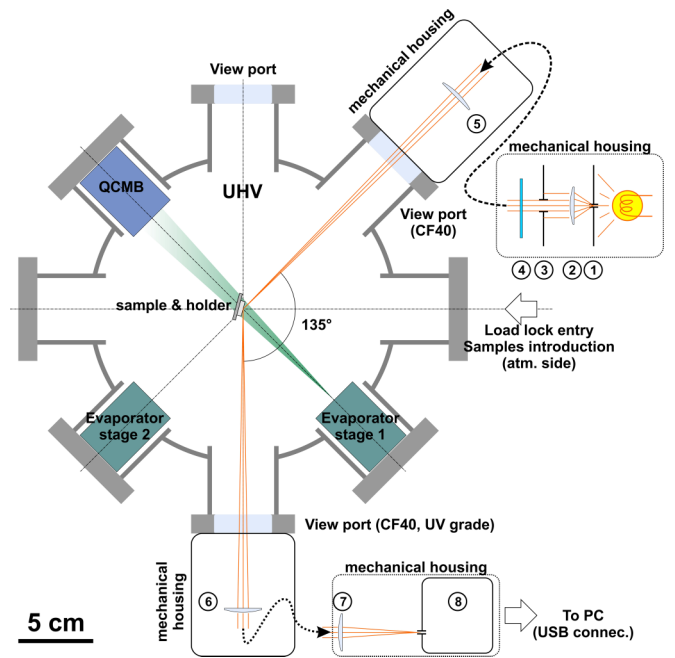
FIG. 15. Sketch of DRS setup implemented on our UHV chamber, to scale.
