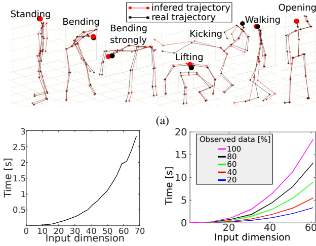
(b) Time to compute movement distributions from 10 trajectory continuation. (c) Time to infer the movement from 10 trajectory continuation. demonstrations.
