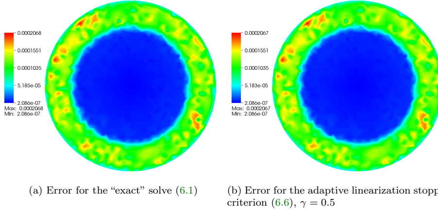
Fig. 8: Comparison of the total errors for different resolution strategies at the final time
