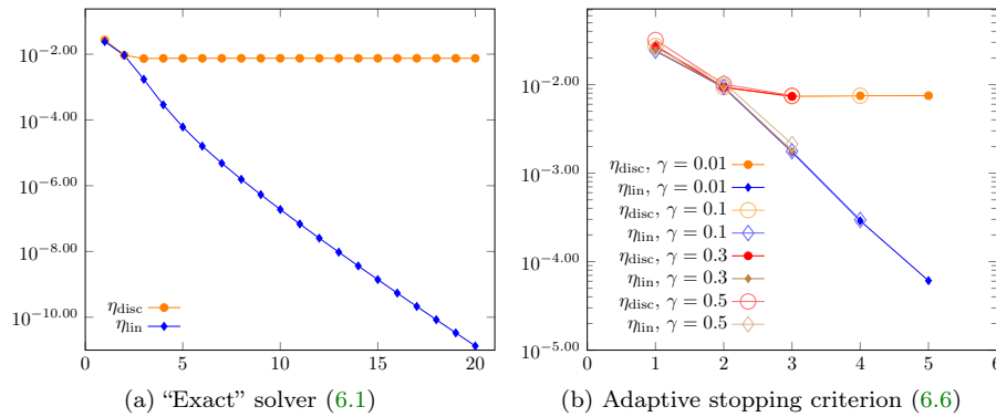
Fig. 7: Linearization and discretization estimators in functions of Newton iterations
