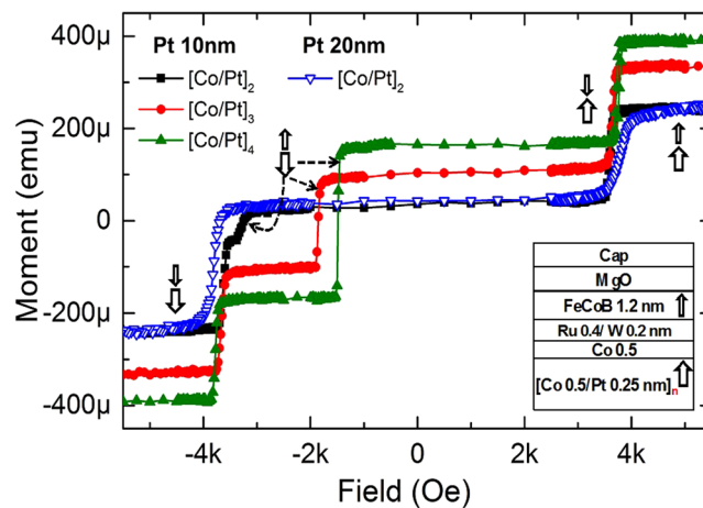
Figure 6. Descending branch of M(H) loops of thin-pSAFs with configuration of Si/SiO 2 500/Ta 3/Pt 10 or 20/[Co 0.5/Pt 0.25] n HIL /Co 0.5/Ru 0.4/W 0.2/FeCoB 1.2/MgO/cap layers (thicknesses are in nm) with different number of Co/Pt bilayers, ( n_{\text{HIL}} = 2, 3 and 4) after annealing at 340 °C. The arrows indicate the magnetization reversal process of the pSAF layers when the magnetic field is swept out-of-plane from +6 kOe to -6 kOe.
