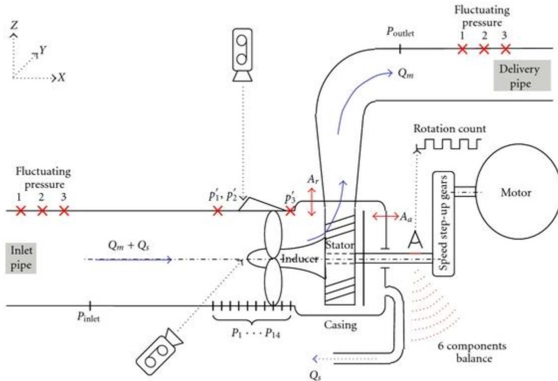
Figure 1. Scheme of the pump test rig showing especially the pressure transducers locations in the inlet and outlet pipes
