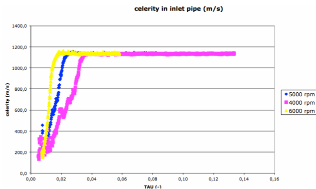
Figure 7. Evolutions of waves celerity in inducer inlet pipe in function of non-dimensional available NPSP for three different speeds of inducer rotation and the same relative flow rate
