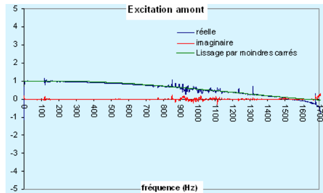
Figure 4. Real (in blue) and imaginary (in red) parts of left side of equation (a) in a stainless steel pipe (inlet diameter = 40 mm; wall thickness = mm) at inlet of a radial flow pump as functions of frequency (in abscissa). Green curve represents the “ \cos kL ” function that optimally approximates the real part of experimental results. From that green curve, wave celerity of 1270 m/s is deduced.
