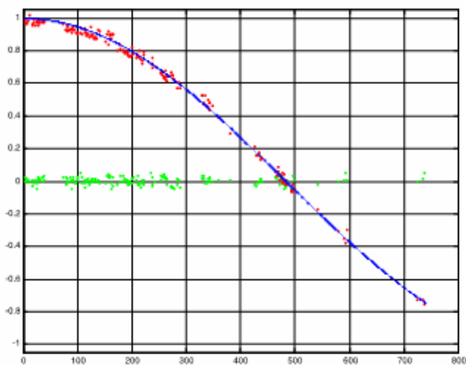
Figure 5. Real (red points) and imaginary (green points) of the left side of equation (a). Evolutions with frequency (Hz, in abscissa) for one time window (duration 2 s) during a transient cavitation test of an inducer. Blue lines represent the “coskL” function fitted to red points and used for the determination of instantaneous waves celerities. Results in inlet pipe (figure on the left) and in outlet pipe (figure on the right)
