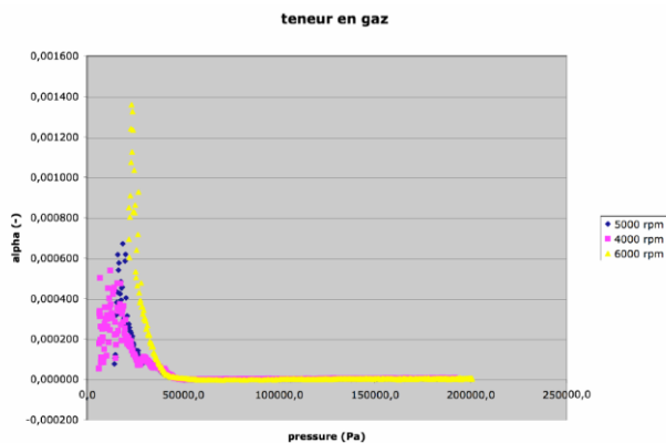
Figure 9. Evolutions with available NPSP of inlet pipe gas content calculated from celerity in Figure 8
