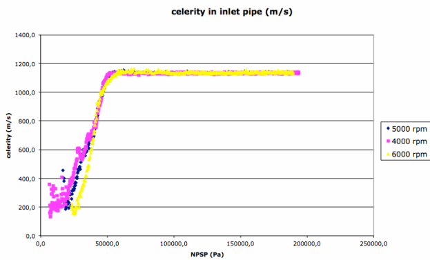
Figure 8. Evolutions of waves celerity in inducer inlet pipe in function of available NPSP for three different speeds of inducer rotation and the same relative flow rate
