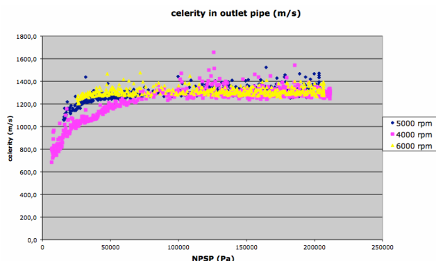
Figure 10. Evolutions of celerity in outlet pipe with NPSP
