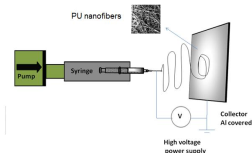
Figure 3. Schematic illustration of the nanofiber electrospinning process
