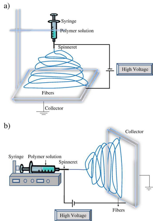
Figure 2. Schematic diagram of set-up of electrospinning a) typical vertical set-up, b) horizontal set up [4]
