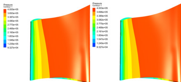
(a) (b) Figure 7. Pressure side static pressure contour map: (a) coupledFoam upper, (b) LINARS.
