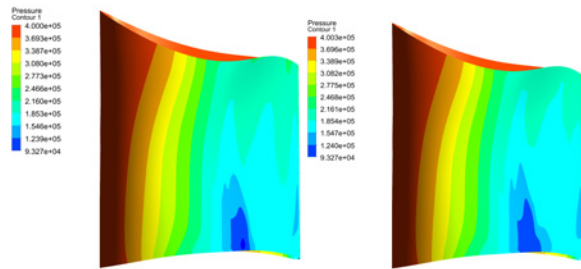
(a) (b) Figure 8. Suction side static pressure contour map a) coupledFoam, b) LINARS
