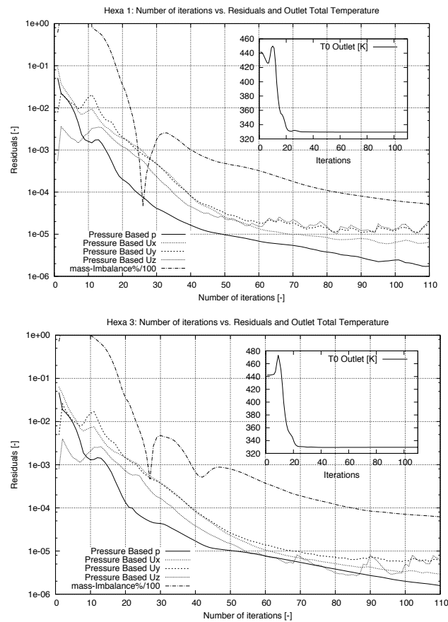
Figure 10. Residuals, total temperature and mass imbalance convergence for the pressure-based solver
