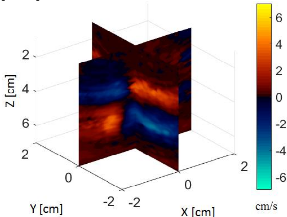
Fig. 5. 1D Doppler velocity components for the x - z and y - z planes
