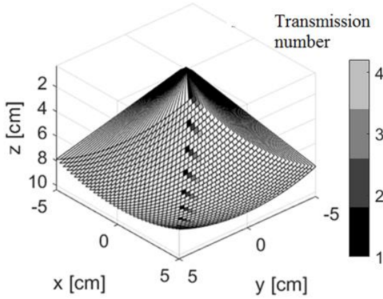
Fig. 2. Transmission scheme for 8 MLT along the transverse diagonal of the transducer
