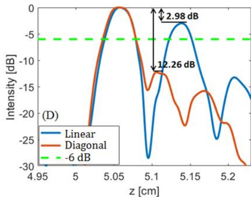
Fig. 4. Axial profiles at the center of the XZ (A) and YZ (C) planes, and their corresponding zoomed regions (B, D), after normalizing the region of interest (black rectangle) between [-60, 0] dB. The difference between the main and the side lobe is shown for each case.
