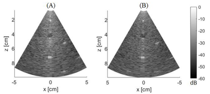
Fig. 5. Comparison between the 8 MLT Gammex phantom results using the linear transmission scheme (left) and the diagonal transmission scheme
