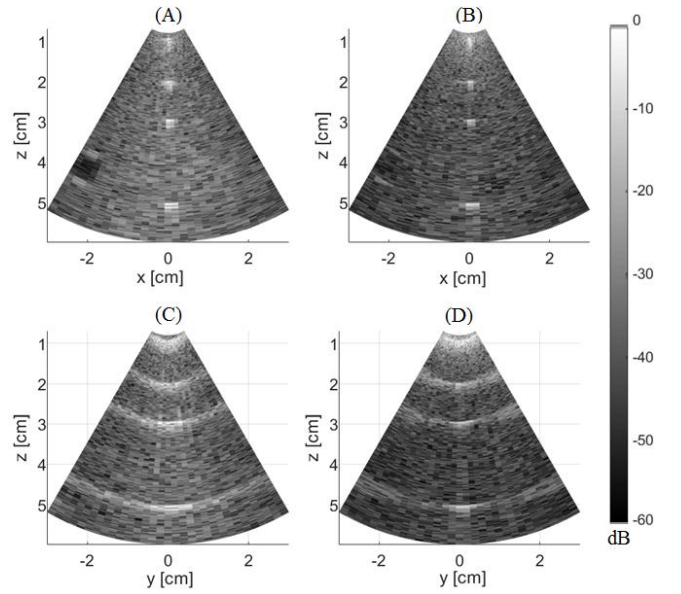
Fig. 3. Comparison between the 8 MLT Gammex phantom results using the linear transmission scheme (left) and the diagonal transmission scheme (right) for both XZ (A, B) and YZ planes (C, D).
