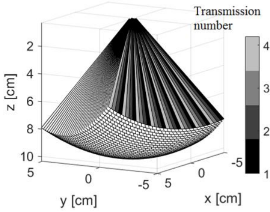
Fig. 1. Linear transmission scheme for 8 MLT
