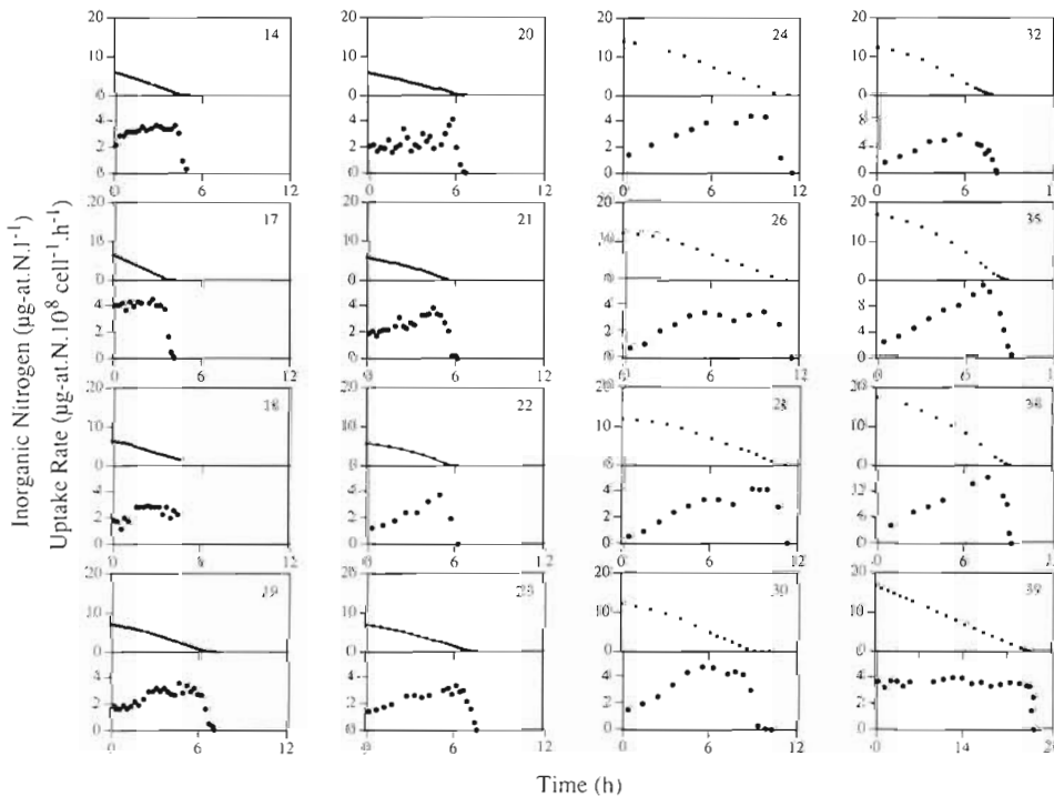
Fig. 3. Time variation of inorganic nitrogen (■) and uptake rate of Prococtrum minimum (●) following nitrate additions. Numbers in right-hand corner indicate the day of the pulsed experiments. Note difference in uptake scales for Days 32, 35 and 38
