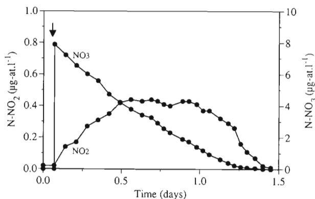
Fig. 5. Changes in nitrate and nitrite in a chemostat culture of nitrate-limited cells of Prorocentrum minimum following a nitrate addition
