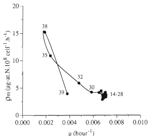
Fig. 7. Prorocentrum minimum . Time changes in growth and uptake rates during the pulsed phase. The 2 processes become largely uncoupled for the 3 d pulsed phase. Numbers indicate pulsed experiment days
