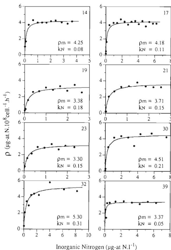
Fig. 4. Prorocentrum minimum . Nitrogen uptake kinetics obtained from perturbation experiments during which cells sustained a stable uptake rate before limitation due to nutrient deprivation. Numbers in right-hand corner indicate day of pulsed experiments
