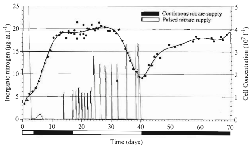
Fig. 1. Time variation of Prorocentrum minimum (dots and fitted curve) and inorganic nitrogen concentration (thin line) in the chemostat. During the pulsed phase (except during the first pulse), the continuous inflow medium was deprived of nitrate
