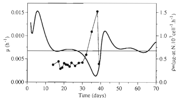
Fig. 2. Prorocentrum minimum . Continuous line: growth rate during the 70 d time-course experiment. Line with data points: maximum uptake rates measured during each pulsed experiment. Horizontal line represents dilution rate
