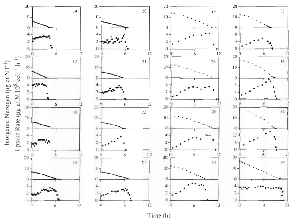
Fig. 3. Time variation of inorganic nitrogen (■) and uptake rate of Prorocentrum minimum (●) following nitrate additions. Numbers in right-hand corner indicate the day of the pulsed experiments. Note difference in uptake scales for Days 32, 35 and 38
