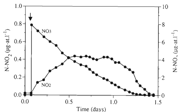
Fig. 5. Changes in nitrate and nitrite in a chemostat culture of Prorocentrum minimum following a nitrate addition
