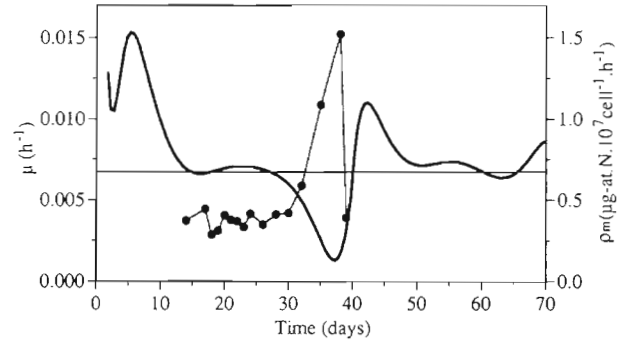
Fig. 2. Prococtrum minimum . Continuous line: growth rate during the 70 d time-course experiment. Line with data points: maximum uptake rates measured during each pulsed experiment. Horizontal line represents dilution rate
