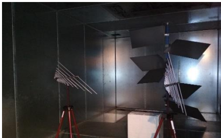
Fig. 2. IETR's reverberation chamber with the two log-periodic antennas and the three masts.
