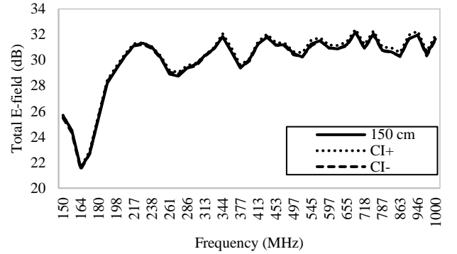
Fig. 9. Total E-field for d = 150 cm compared with the confidence interval.
