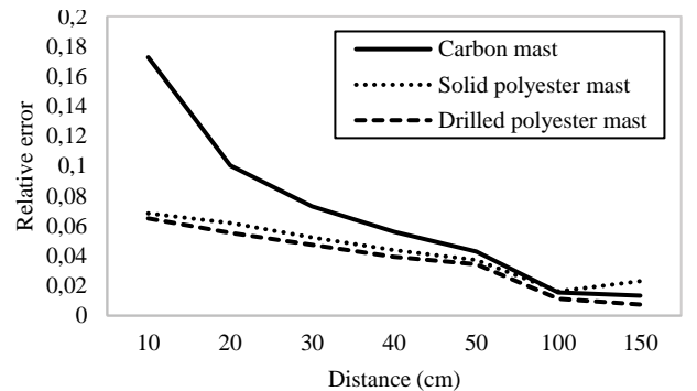
Fig. 11. Relative error between the total electric field amplitude with and without the three masts over the frequency range 150 – 1000 MHz as a function of the mast-field probe distance.
