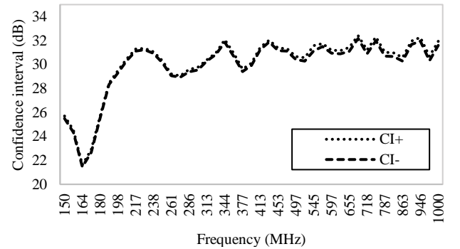
Fig. 7. Confidence interval in the empty chamber.
