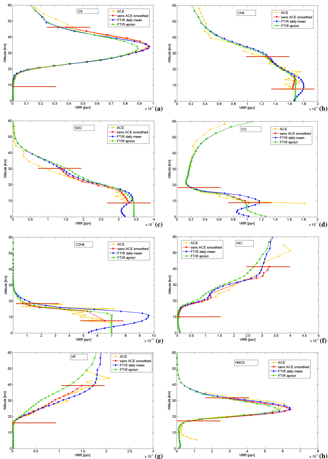
Fig. 14. Vertical vmr profiles from 0 to 60 km of (a) O 3 on 4 October, (b) CH 4 on 20 August, (c) N 2 O on 4 October, (d) CO on 4 October, (e) C 2 H 6 on 6 October, (f) HCl on 4 October, (g) HF on 20 August, and (h) HNO 3 on 20 August, measured at St.-Denis in 2004 by ground-based FTIR (blue diamonds) and by ACE-FTS (raw: yellow circles; smoothed: red stars). The FTIR a priori profile is indicated by the green triangles.
