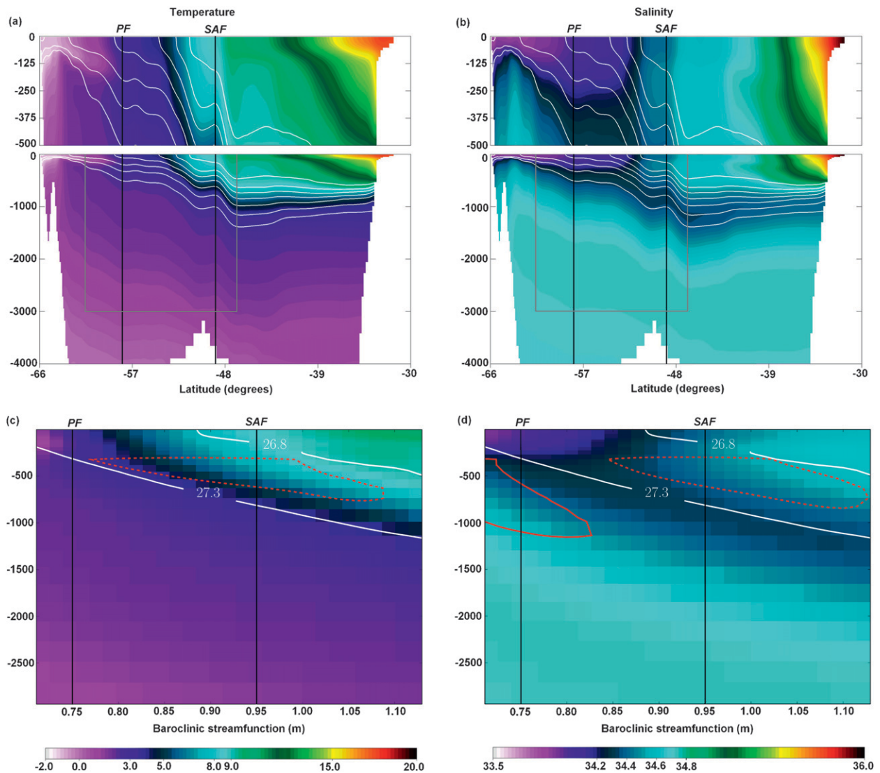
FIG. 1. Mean (a),(c) potential temperature and (b),(d) salinity cross section along 130^{\circ}\text{E} , in the DRACKAR model. (a),(b) Fields in physical plane (latitude, p ), a zoom on the upper 500 m is done; white contours indicate isopycnals ranging from \sigma_0 = 26.8 \text{ kg m}^{-3} to \sigma_0 = 27.4 \text{ kg m}^{-3} with a 0.1 \text{ kg m}^{-3} contour interval. (c),(d) Fields in streamfunction plane ( \phi_{1000-3000}, p ). The latitude band used ranges from 45^{\circ} to 60^{\circ}\text{S} . Color bars indicate potential temperature ( ^{\circ}\text{C} ) and salinity (psu). Continuous and dashed red contours indicate the location of the main anomalies in the EOF analysis (see below). White solid contours indicate the mean position of isopycnal \sigma_0 = 26.8 \text{ kg m}^{-3} and isopycnal \sigma_0 = 27.3 \text{ kg m}^{-3} , respectively.
