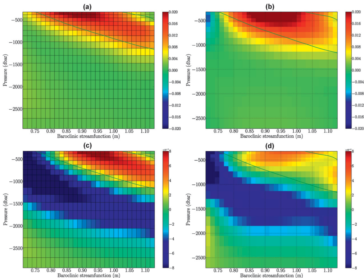
FIG. 4. First DRAKKAR model EOF for (a),(b) potential temperature and (c),(d) salinity within the 300–3000-dbar layer calculated (a),(c) in streamfunction space and (b),(d) in physical space then projected into streamfunction space. The latitude band used ranges from 45^{\circ} to 60^{\circ} S. Green lines indicate isopycnals \sigma_0 = 26.8 \text{ kg m}^{-3} (upper line) and 27.3 \text{ kg m}^{-3} (lower line).
