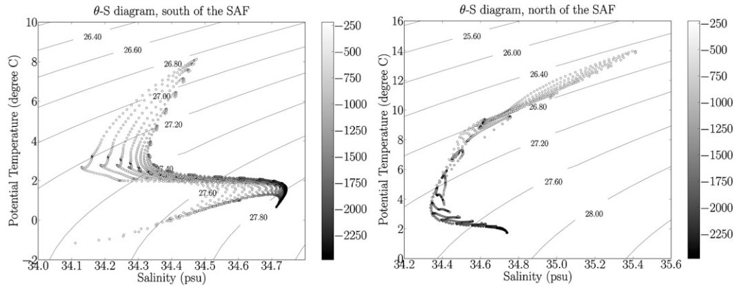
FIG. 2. Subsampled temperature–salinity diagram (left) south and (right) north of the SAF along 130°E for a latitude ranging from 30° to 66°S in the DRAKKAR model, showing the thermohaline properties averaged over 25 yr (1980–2004). A \theta – S point is drawn for each grid point of the model located between a depth of 200 and 2500 m along 130°E and whose surface-referenced potential density ranges from \sigma_0 = 26.5 \text{ kg m}^{-3} to \sigma_0 = 28.0 \text{ kg m}^{-3} . The SAF is located at 49°S. Gray shades on the vertical bar represent the depth (dbar), and the background contours indicate isopycnals ( \text{kg m}^{-3} ).
