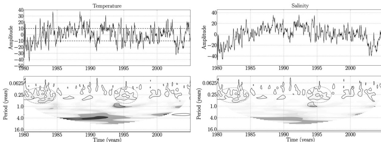
FIG. 5. First EOF temperature and salinity time series (arbitrary units) for (top) the 300–3000-dbar layer and (bottom) their wavelet transforms. The latitude band used ranges from 45^{\circ} to 60^{\circ} S. The shaded contours are at normalized variances of 0, 2, 5, 10, 15, 20, 50, and 70. The dashed lines that appear at amplitudes of 10 and -10 on the first EOF temperature time series represent the \pm 0.8 standard deviation threshold chosen for building the composite time series used in the study of positive and negative phases of the pulsation mode.
