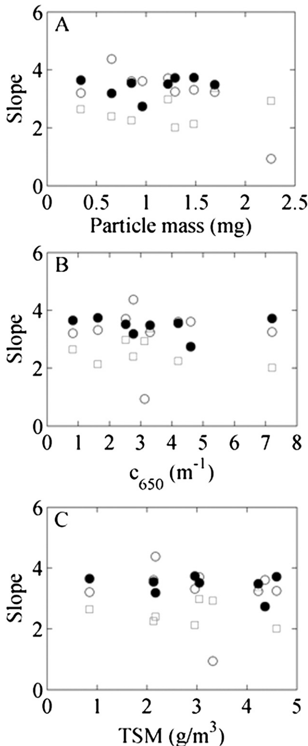
FIG. 7. Comparison of slopes calculated for particle diameters from 2 to approximately 10 \mu\text{m} from SEM analysis (open circles), LISST-100X (open squares), and 30- \mu\text{m} Elzone (black filled circles) for Long Island Sound samples as a function of mass on (a) the filter, (b) c_{650} , and (c) TSM.
