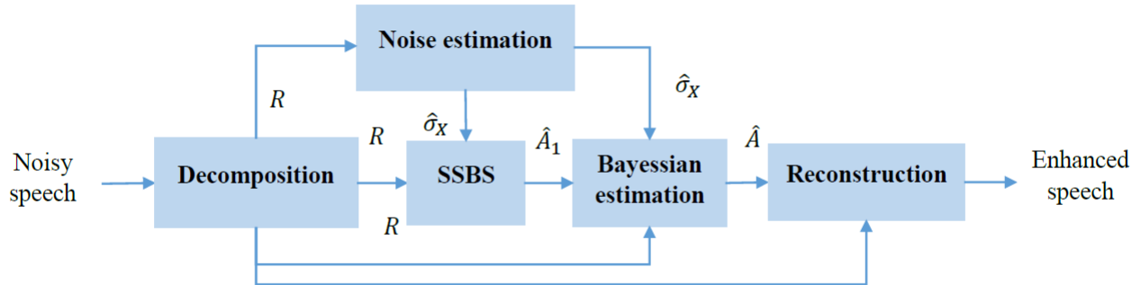
Fig. 1. Processing chain of the proposed algorithm using a smoothed rough binary masking
