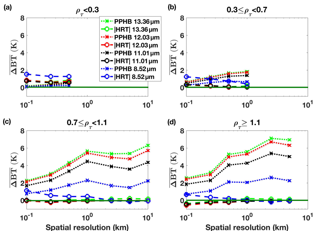
Figure 10. Scene-average, plane-parallel and homogeneous bias (PPHB) and mean deviation due to the horizontal radiative transport ( |HRT| ) effect on brightness temperatures ( \Delta BT ) for (a) small, (b) medium, (c) large and (d) very large pixel inhomogeneity ( \rho_\tau ) as a function of spatial resolution in channels centered at 8.52, 11.01, 12.03 and 13.36 \mu\text{m} . The small optical thickness range corresponds to 8969 pixels, the 2724 medium pixels, the 347 large pixels and the 89 very large pixels.
