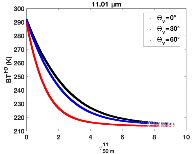
Figure 11. One-dimensional brightness temperatures as a function of the 50 m optical thickness \tau_{50\text{m}}^{1\text{-D}} for viewing zenith angles \Theta_v = 0, 30 and 60^\circ at a constant view azimuth angle of 0^\circ .
