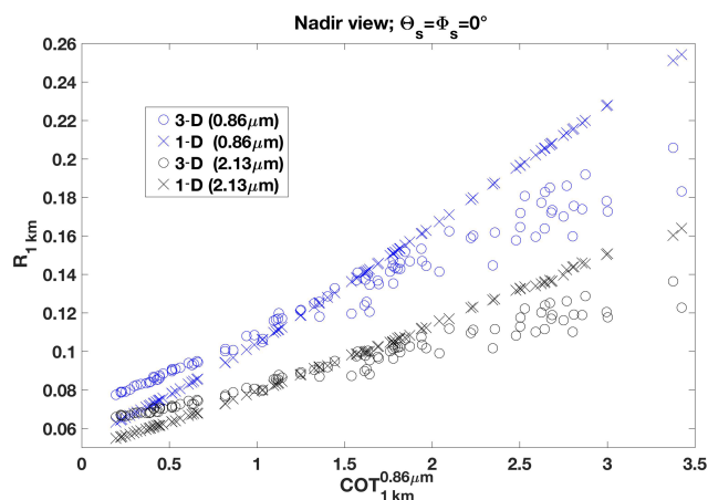
Figure 5. Solar reflectances at 0.86 \mu\text{m} (blue) and 2.13 \mu\text{m} (black) at 1 \text{ km} spatial resolution computed in 3-D (circles) and in 1-D (crosses). We choose to show these reflectances at 1 \text{ km} to not overload the plot with too many points at finer spatial resolutions, but the effect is the same.
