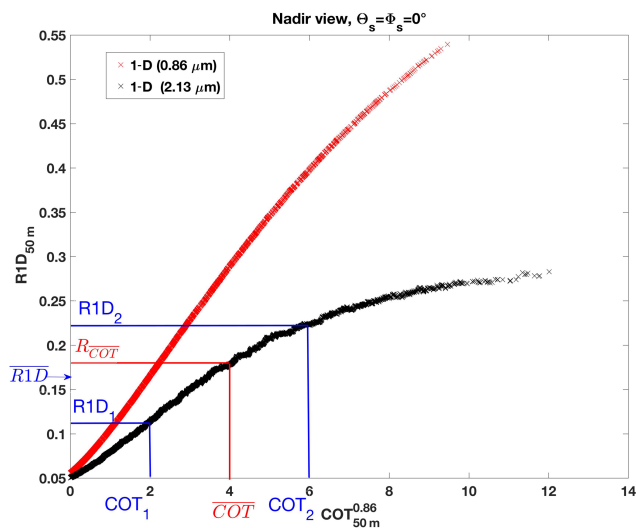
Figure 3. 1-D reflectances ( R_{50m}^{1D} ) as a function of the 50 m optical thickness at 0.86\ \mu\text{m} ( COT_{50m}^{0.86\ \mu\text{m}} ) for channels centered at 0.86\ \mu\text{m} (red) and 2.13\ \mu\text{m} (black) for nadir view and overhead Sun. R_{1D_1} and R_{1D_2} represent the reflectances corresponding to the optical thicknesses COT_1 and COT_2 , respectively, and COT is their averaged value. Because of the nonlinearity between R_{1D} and COT , the average reflectance \overline{R_{1D}} is smaller than the reflectance of the average optical thickness R_{COT} .
