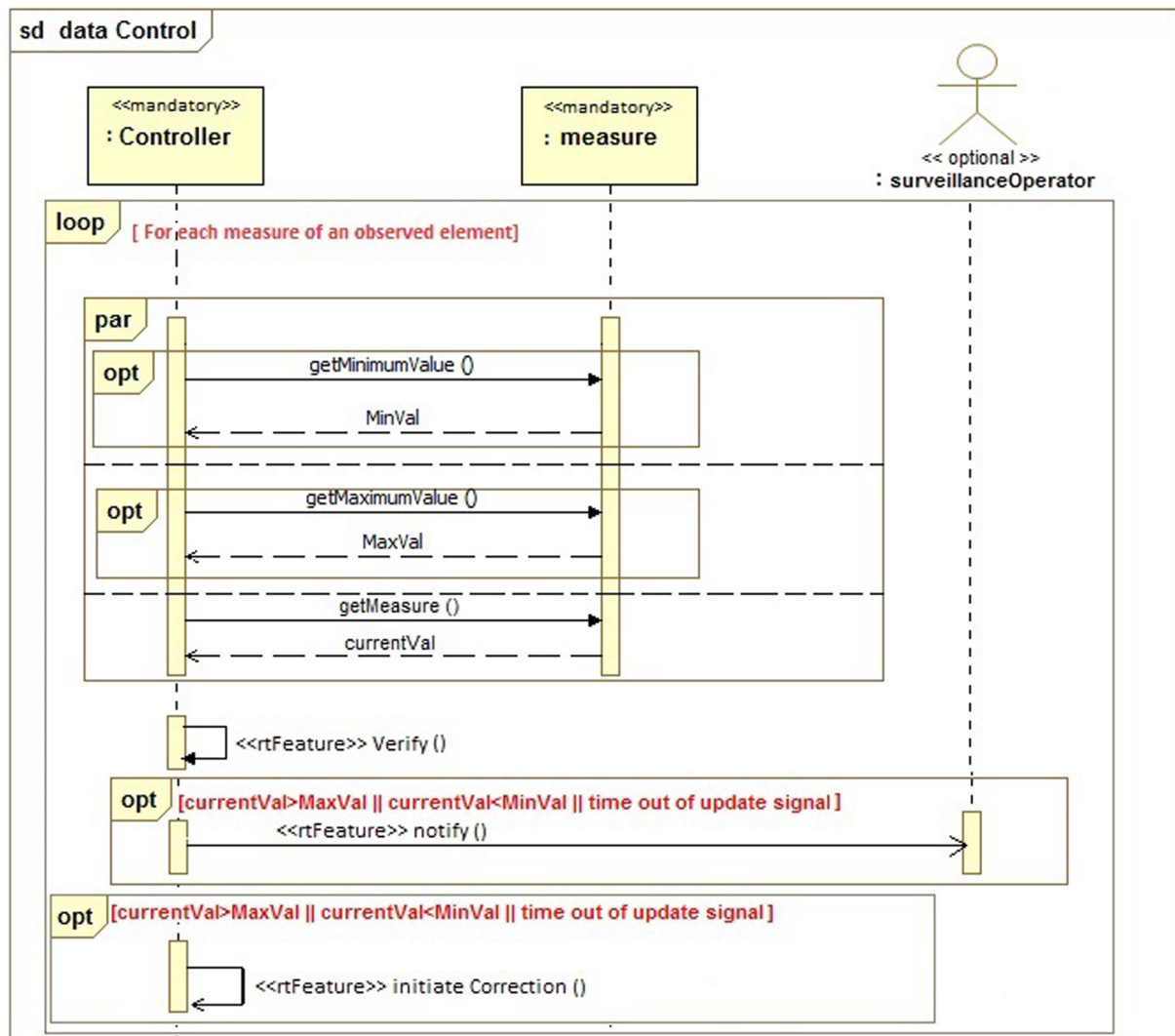
Figure A8 Sequence diagram of RT controller pattern.
