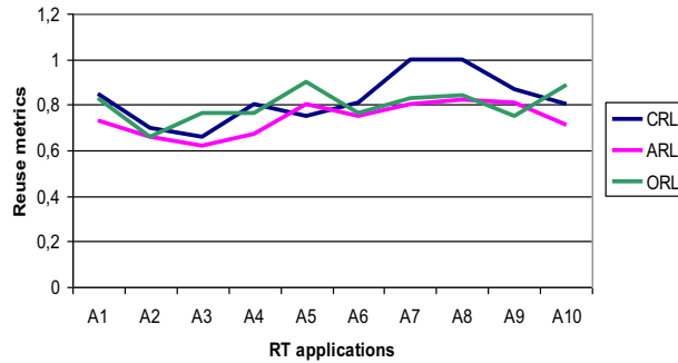
Figure 8 Evaluation of RT design patterns based on reuse metrics.
