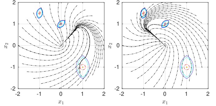
Fig. 7. (Example VII-C) Closed-loop solutions for the perturbed system dynamics w_1 (left) and w_2 (right) defined in (39) and (40), respectively.
