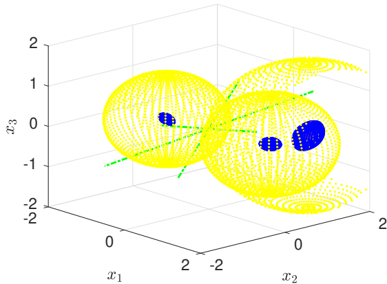
Fig. 8. (Example VII-D) Visualization of the shells S_{h_i}^i(\delta_i^*) (blue), the \eta_i -balls (yellow) and the subspaces \mathcal{E}_i (green) for i = 1, 2, 3 .
