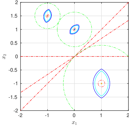
Fig. 4. (Example VII-A; Setting) Visualization of the setting for the unsafe points \hat{x}_1, \hat{x}_2, \hat{x}_3 . The shells \mathcal{S}^i(\delta_i) (blue) and \mathcal{S}^h(\delta_i) (cyan), the \eta_i -balls (green) and the subspaces \mathcal{E}_i (red) are shown. The balls \mathcal{B}_{\frac{h_i \mu_i \delta_i}{4}}(\hat{x}_i) for which avoidance is guaranteed are depicted in red.
