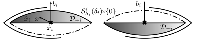
Fig. 3. The upper and lower half-shells associated to \mathcal{D}_{+i} = (\mathcal{S}_{h_i}^i(\delta_i) \cap \mathcal{F}_{+1}^i) \times \{0\} and \mathcal{D}_{-i} = (\mathcal{S}_{h_i}^i(\delta_i) \cap \mathcal{F}_{-1}^i) \times \{0\} , respectively, in (25), for an arbitrary unsafe point \hat{x}_i , i \in \mathbb{N}_\beta .
