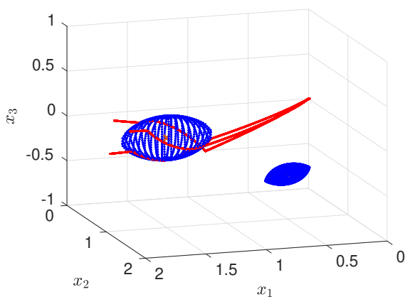
Fig. 9. (Example VII-D) Visualization of closed-loop solutions of the avoidance controller for a three dimensional example focusing on the unsafe point \hat{x}_2 . Depending on the initial state, the obstacle is passed by sliding along the surface of the upper or lower shell (with respect to the orientation b ).
