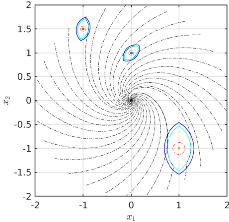
Fig. 5. (Example VII-A; Closed-loop solutions) Visualization of 50 closed-loop solutions avoiding a pre-specified neighborhood around the unsafe points \hat{x}_1, \hat{x}_2, \hat{x}_3 , and converging to the origin.
