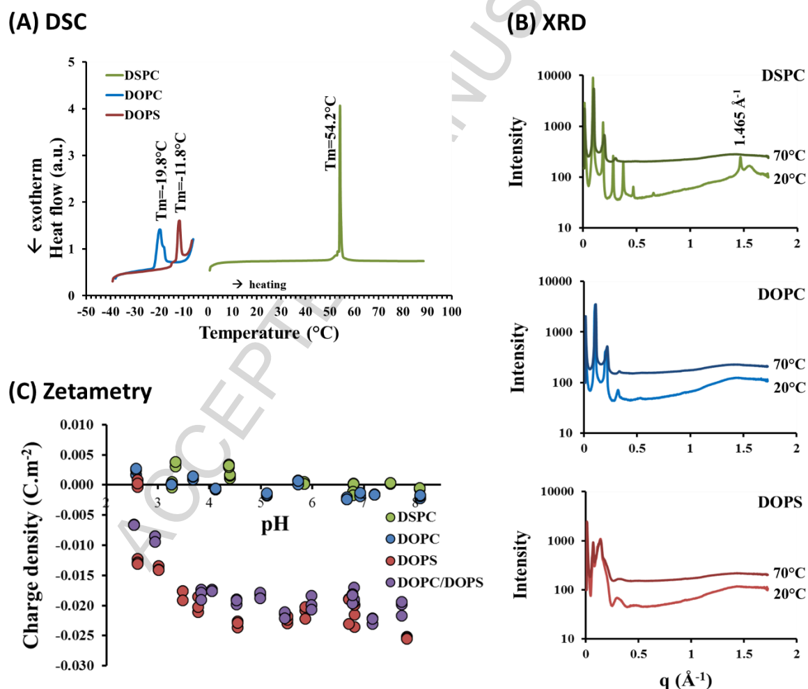
Figure 3. Physical properties of bilayers of DSPC, DOPC and DOPS in PIPES/ NaCl/0.1 mM \text{CaCl}_2 buffer at pH 6.7. (A) Determination of T_m by DSC upon heating MLVs at 2^\circ\text{C}\cdot\text{min}^{-1} . (B) X-ray Scattering spectra of MLVs recorded at 20 or 70^\circ\text{C} at Wide ( q > 1 \text{ \AA}^{-1} ) and Small angles ( q < 0.5
