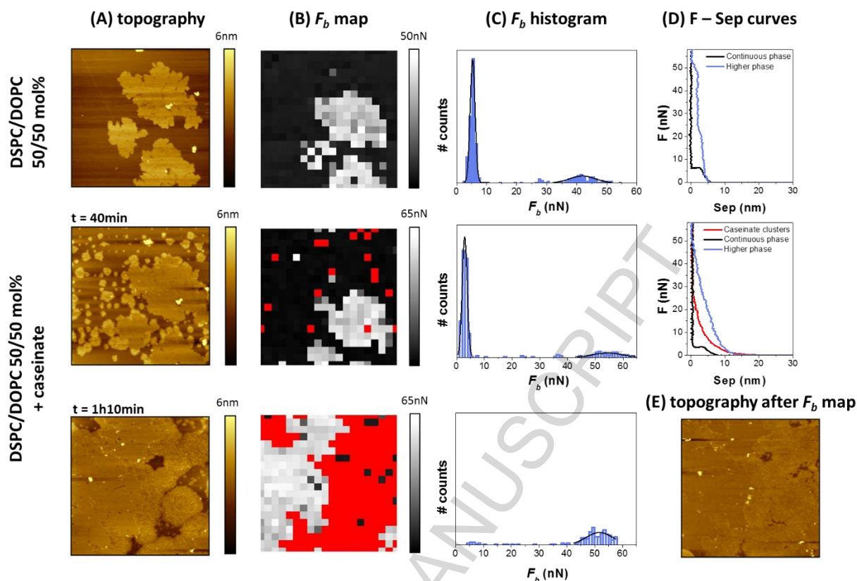
Figure 5. Change in mechanical stability of DSPC/DOPC 50/50 mol% bilayers as a consequence of adsorption of sodium caseinate, measured by AFM-FS in PIPES/NaCl/0.1 mM CaCl 2 buffer at pH 6.7 and at 20°C. (A) AC mode topography over 8×8 μm 2 , (B) corresponding F_b maps, (C) F_b histogram and (D) typical force-separation curves recorded prior to (upper row) or after incubation for 40 min (middle row) or for 1h10min (bottom row) in presence of sodium caseinate. (E) A different location (5×5 μm 2 ) after performing the F_b map. Red pixels on the F_b maps indicate the absence of a breakthrough event.
