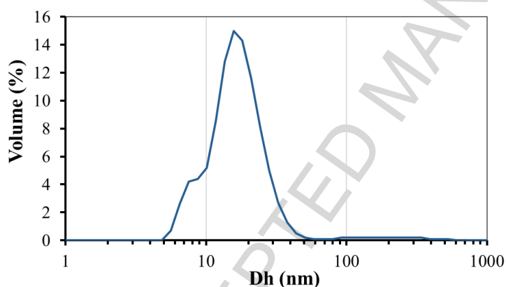
Figure 2. Average dynamic light scattering distribution in volume of the hydrodynamic diameter D_h of 1 \text{ mg}\cdot\text{mL}^{-1} sodium caseinate in PIPES/NaCl/0.1 mM \text{CaCl}_2 buffer at pH 6.7 and at 20^\circ\text{C} .
