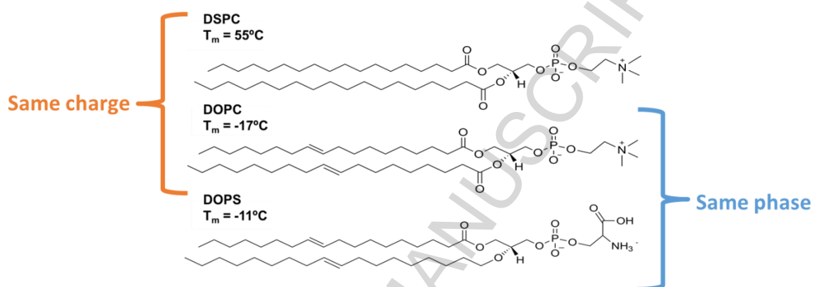
Figure 1. Molecular structures and indicative melting temperatures ( T_m ) of 1,2-distearoyl- sn -glycero-3-phosphocholine (DSPC), 1,2-dioleoyl- sn -glycero-3-phosphocholine (DOPC) and 1,2-dioleoyl- sn -glycero-3-phosphoserine (DOPS - Avanti Polar Lipids).
