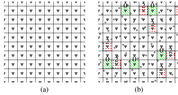
Fig. 2: (a) Points of \mathbb{Z}^2 (triangles), initially located at the center of unit squares of the Cartesian tiling of the Euclidean space. (b) After a rigid motion \mathcal{T} of these points (circles), some of the unit square cells contain no point (non-surjectivity, green cells) or two points (non-injectivity, red cells); the transformation \mathcal{T} is no longer bijective.
