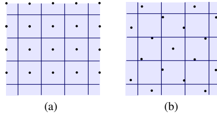
Fig. 2. (a) Points of \mathbb{Z}^2 , initially located at the center of unit squares of the Cartesian tilling of the Euclidean space. (b) After a rigid motion \mathfrak{T} of these points, some of the unit square cells contain no point (non-surjectivity) or two points (non-injectivity); the transformation \mathcal{T} is no longer bijective.
