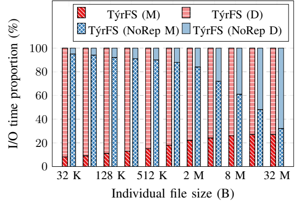
Fig. 7. Breakdown of reads between metadata (M) and data (D) access for a fixed-size data set varying the size of the individual files it is composed of.
