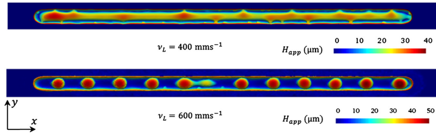
Fig. 6. Colour map of single-track height H_{app} (with respect to the substrate surface) with different scanning speeds v_L . The track length is 2.6 mm.
