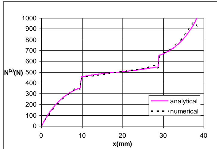
Figure 9. Comparison between numerical and analytical approaches ( b=1\text{mm} , C_u=10000\text{N/mm} )
