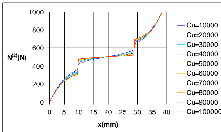
Figure 8. Load transfer as a function of C_u ( b=1\text{mm} )
