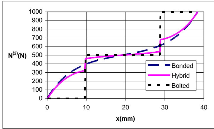
Figure 7. Load transfer ( b=1\text{mm} , C_u=40000\text{N/mm} )
