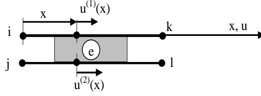
Figure 6. Bonded-bar element
