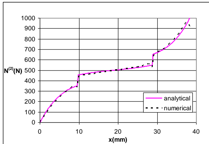
Figure 9. Comparison between numerical and analytical approaches ( b=1mm , C_u=10000N/mm )
