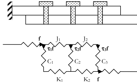
Figure 1. Electric meshing of bolted joint
