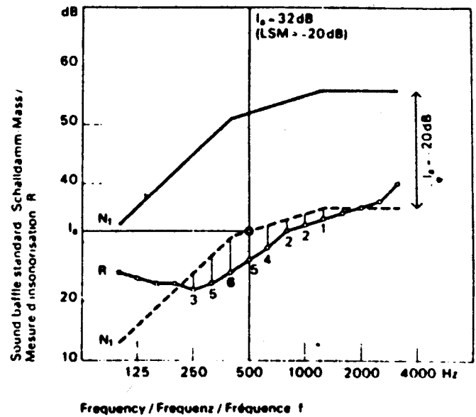
Air-propagated-sound insulation index / Luftschall-Isolationsindex / indice d'isolation phonique I_a
