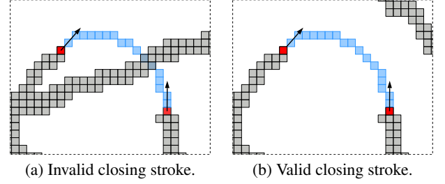
Figure 7: Configurations of stroke closing using a spline in a part of an image I_b (in gray). In (a) the spline curve \mathcal{S} (in blue) between the two key-points (in red) is such that \tau(\mathcal{S}, I_b) = 4 ; it is therefore not added. Note however that the bottom-right stroke may be judiciously extended by a line segment (subsection 5.2). In (b) we have \tau(\mathcal{S}, I_b) = 2 , the curve can therefore be drawn.
