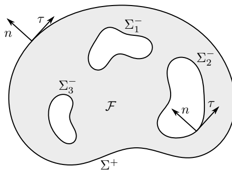
FIGURE 1. The domain of the fluid: an open, \mathcal{C}^{1,1} and N -connected open set.
