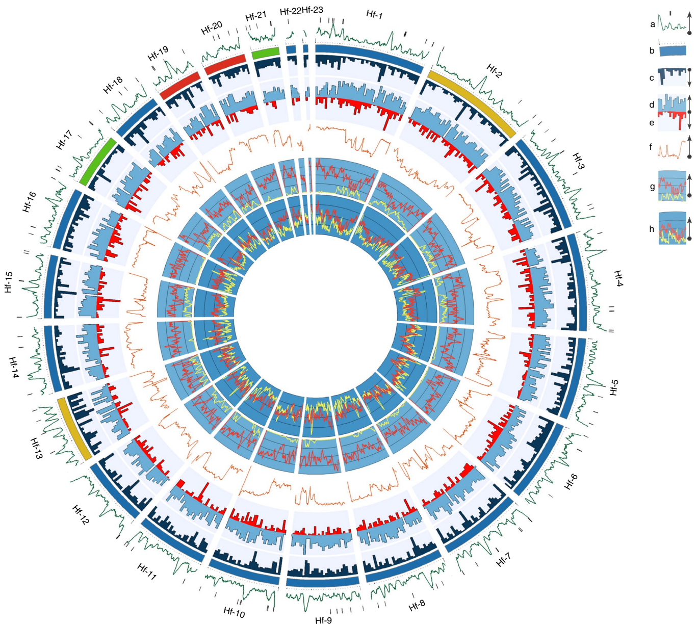
Fig. 2 | H. fraxineus genome organization (scaffolds) and population statistics. a , AT richness sliding window (AT scale = 0.5–0.85; window 63 kbp by 5 kbp slide) with outer ticks indicating gaps in the assembly >2.5 kbp. b , Scaffolds (ticks = 100 kbp) red, green and yellow pairs of scaffolds appear to be from the same linkage group. c , Repeat density (0.0–1.0; 100 kbp). d, e , Gene (blue) and effector (red) density, respectively (0.0–1.0; 100 kbp). f , Genetic differentiation ( F_{ST} ) sliding window between Japanese and European populations (0.01–0.90; 100 kbp by 5 kbp). g , Nucleotide diversity ( \pi ) sliding window within Japanese (red) and European (yellow) populations (0.0–0.032; 100 kbp by 5 kbp). h , SNP density sliding window within Japanese (red) and European (yellow) populations (0.0–0.17; 100 kbp by 5 kbp). Key shows track reference and orientation.
