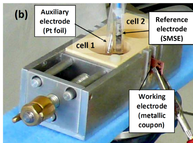
Fig. 2. Electrochemical cell experimental set-up: (a) twin cells prototype (open system – without metallic coupon) and (b) operating device (close system – the metallic coupon is vertically blocked within the two cells).
