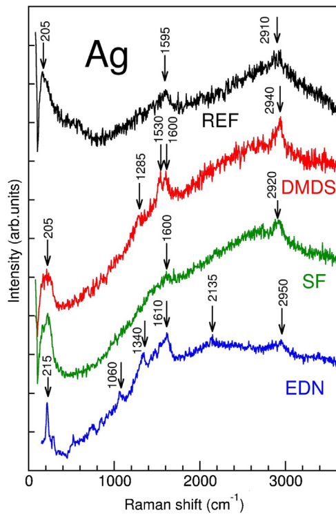
Fig. 7. As measured Raman spectra of silver (Ag) coupons after ageing (488 nm, Ar laser, 0.3 mW).
