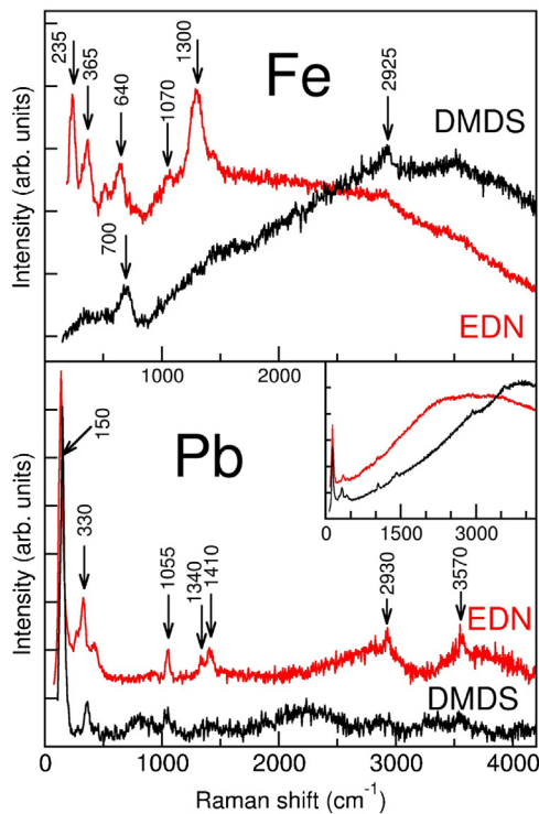
Fig. 8. Raman spectra of iron (Fe) and lead (Pb) coupons after ageing (DMDS and EDN fumigation). Upper part and Inset: raw spectra (488 nm, Ar laser, 0.3 mW). Lead coupons spectra (lower part) are background subtracted.
